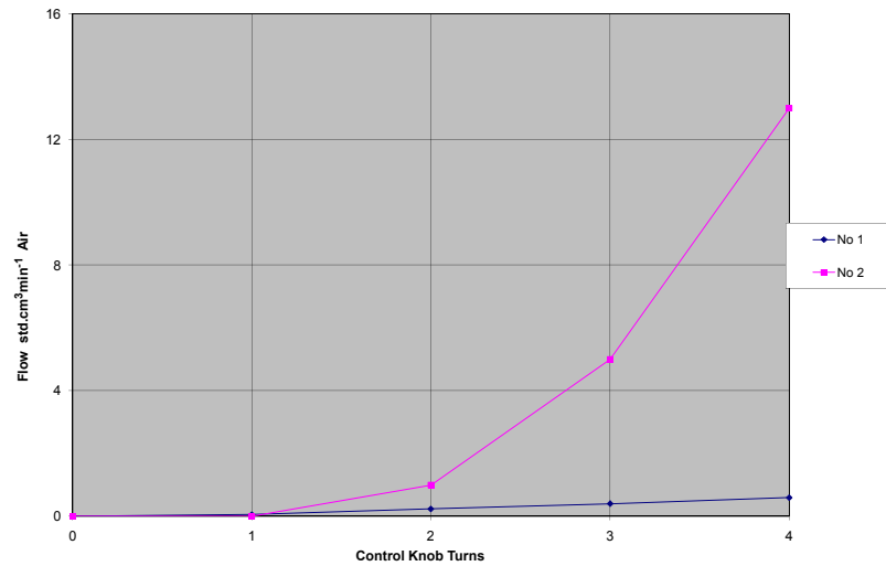
Opening Characteristics, Nos 1 & 2 Needles
