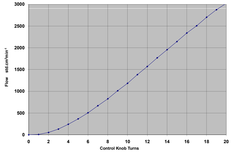
Typical Flow/Turns Plot for No. 3 Needle with 1bar differential Pressure
