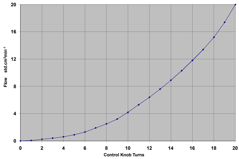
Typical Flow/Turns Plot for No. 1 Needle with 1bar differential Pressure
