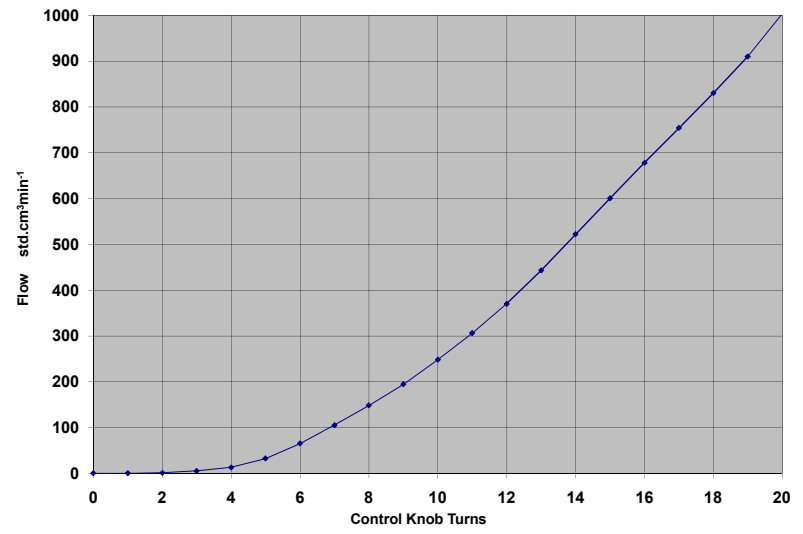
Typical Flow/Turns Plot for No. 2 Needle with 1bar differential Pressure
